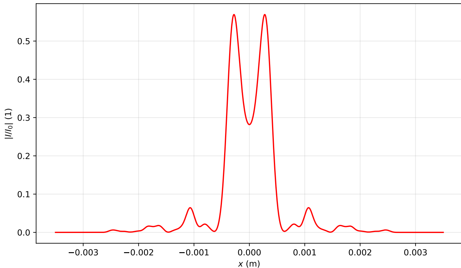
Intensity profile I(x, y = 0, z = 2.149)/I_0 , P_{in}=4.5P_{cr} , artificial time
